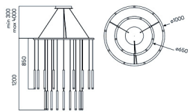
18x3W / 6700lm / 2700K / CRI 80
